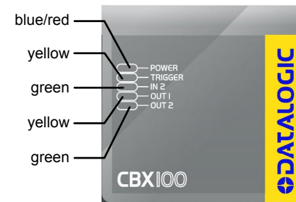
Figure 11 – Indicator LEDs
